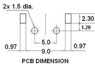
PCB DIMENSION
